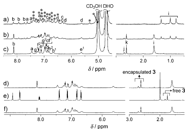
Figure 2. Partial ^1\text{H} NMR spectra (500 MHz, \text{D}_2\text{O}/\text{CD}_3\text{OD} (1:3 v/v), [\mathbf{1}]=2.0 mM, 293 K). a) Box-shaped capsule \mathbf{1}_6 . * denotes \text{H}^a , \text{H}^b , \text{H}^c , and \text{H}^d . b) 0.75 equiv (based on [\mathbf{1}_6] ) of \mathbf{3} was added to a solution of \mathbf{1}_6 . c) Inclusion complex \mathbf{3}@\mathbf{1}_4 obtained upon addition of 1.5 equiv of \mathbf{3} to a solution of \mathbf{1}_6 . d) Dissociation and reconstruction of \mathbf{1}_4 by acid–base control. e) 12 equiv (based on [\mathbf{1}_4] ) of DCl was added to a solution of \mathbf{3}@\mathbf{1}_4 . f) 12 equiv of NaOD was added to the solution in (e).
